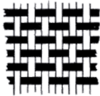
Plain Weave
